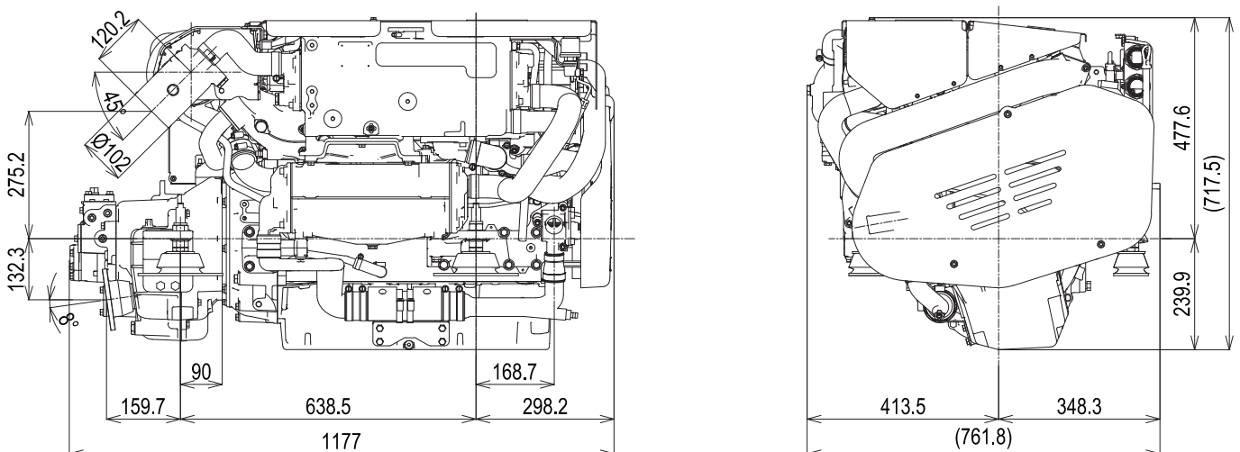
6BY3-260 with KMH51A Marine gear
